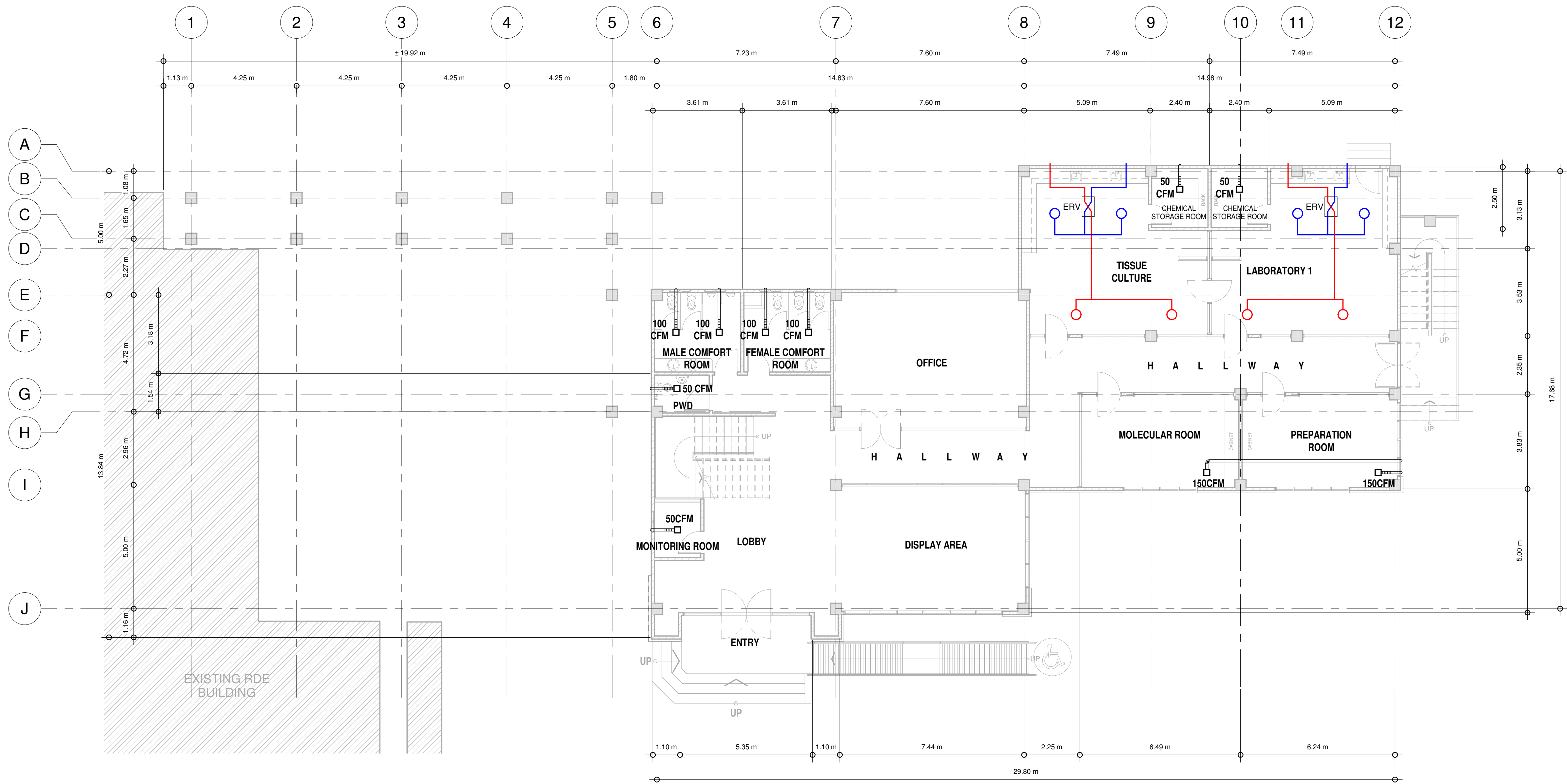
1 GROUND FLOOR EXHAUST FAN LAYOUT PLAN 1 : 100 meters
